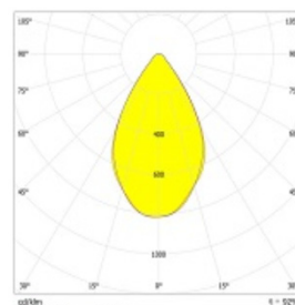
WW VERYWIDE(64°) 8.849lm (147lm/wat)
